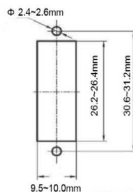
Mounting cutout
