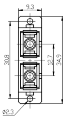
Dimensional drawing
