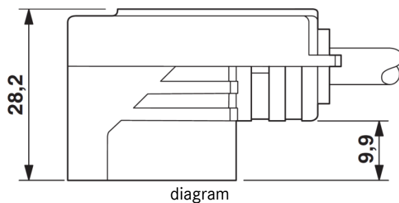
Dimensional drawing
