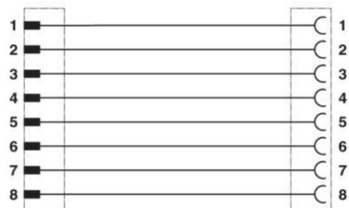
Wiring diagram
