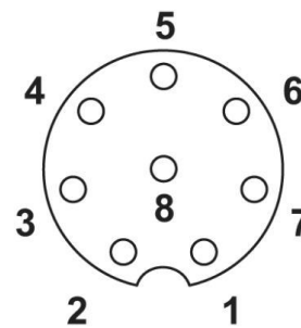
Wiring diagram
