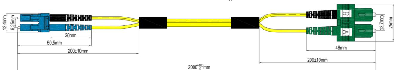
Dimensional drawing
